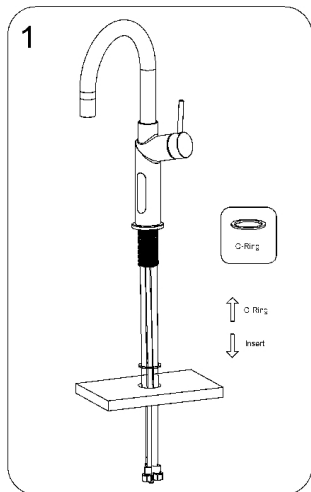
1. Insert the O-ring(B) over the hoses into tap shank, and mount the tap on the sink/Benchtop, see fig.1
